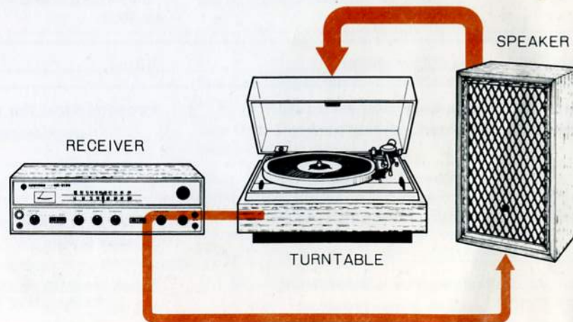
Figure 13. Acoustic Feedback.
