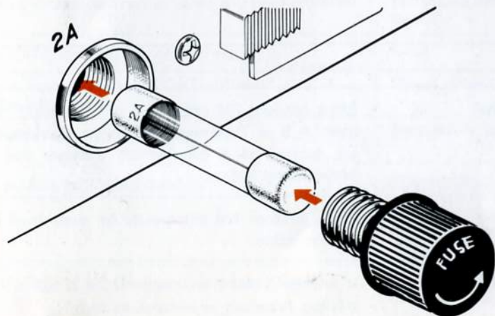
Figure 12. Replace a Fuse.
