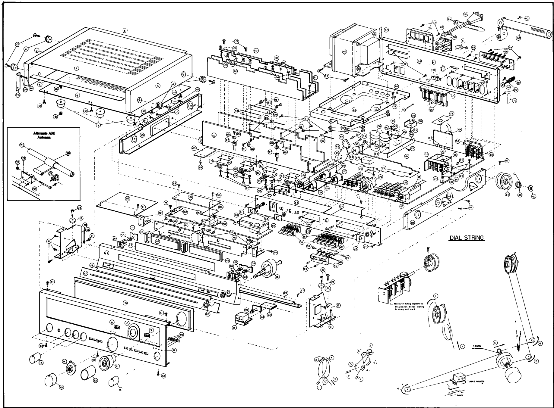
SCOTT 385R EXPLODED VIEW
