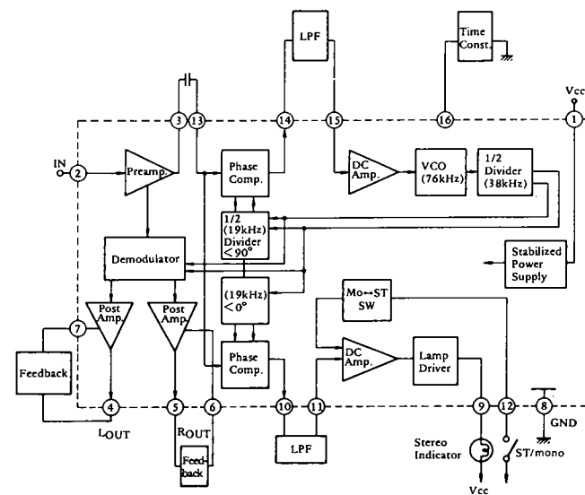
Block Diagram of HA1196 Multiplex Decoder
