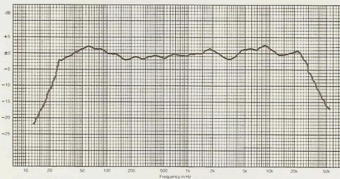
Frequency response of the CONCEPT CE-Monitor
