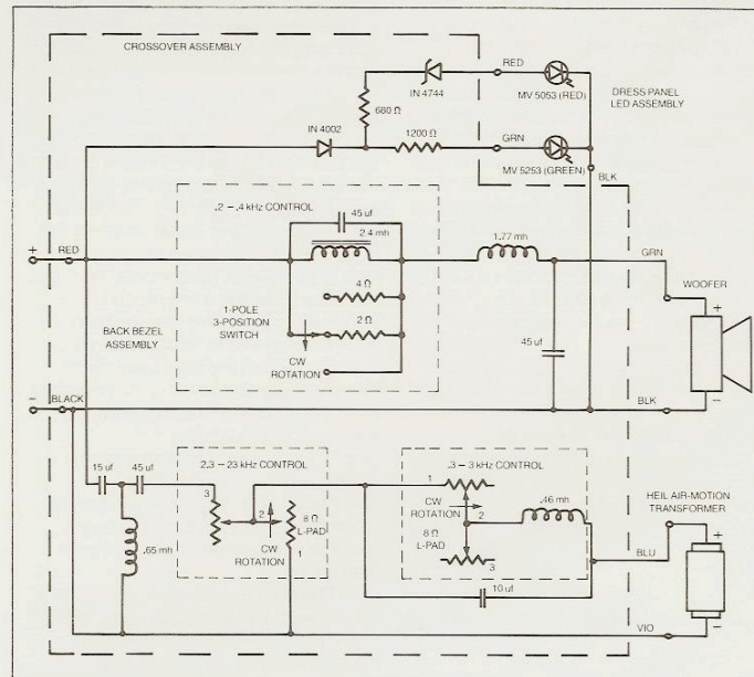
CE-Monitor crossover network schematic
