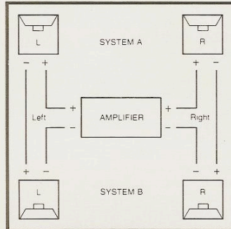
Series speaker connection
