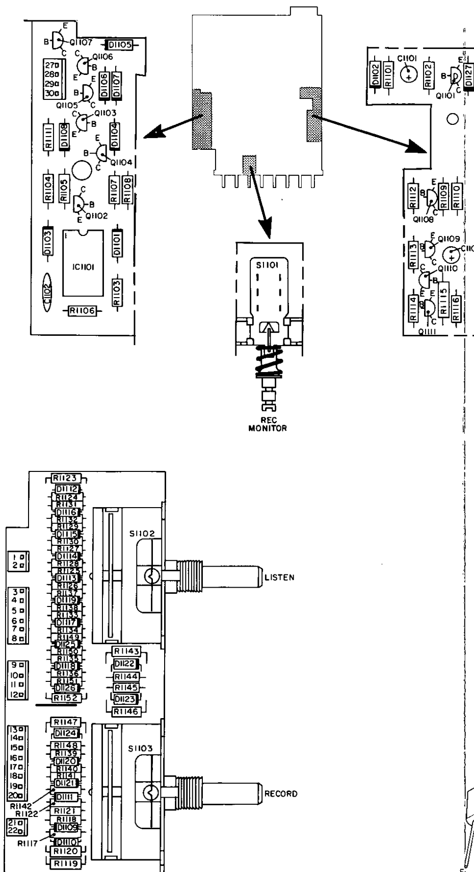
Fig. 11-2. PARTS LOCATION - PC board 045821.
