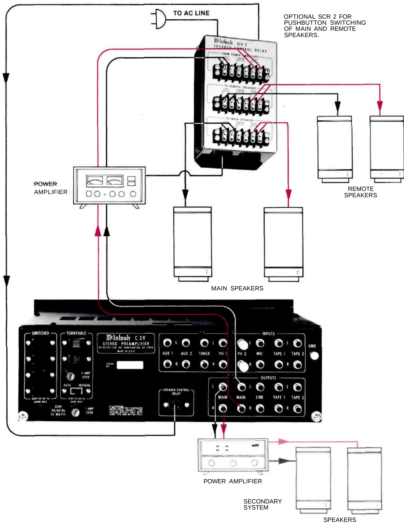
CONNECTIONS FOR POWER AMPLIFIERS AND LOUDSPEAKERS
