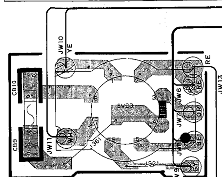
RX-460/360 MAIN P. C. B. ( 9 )
