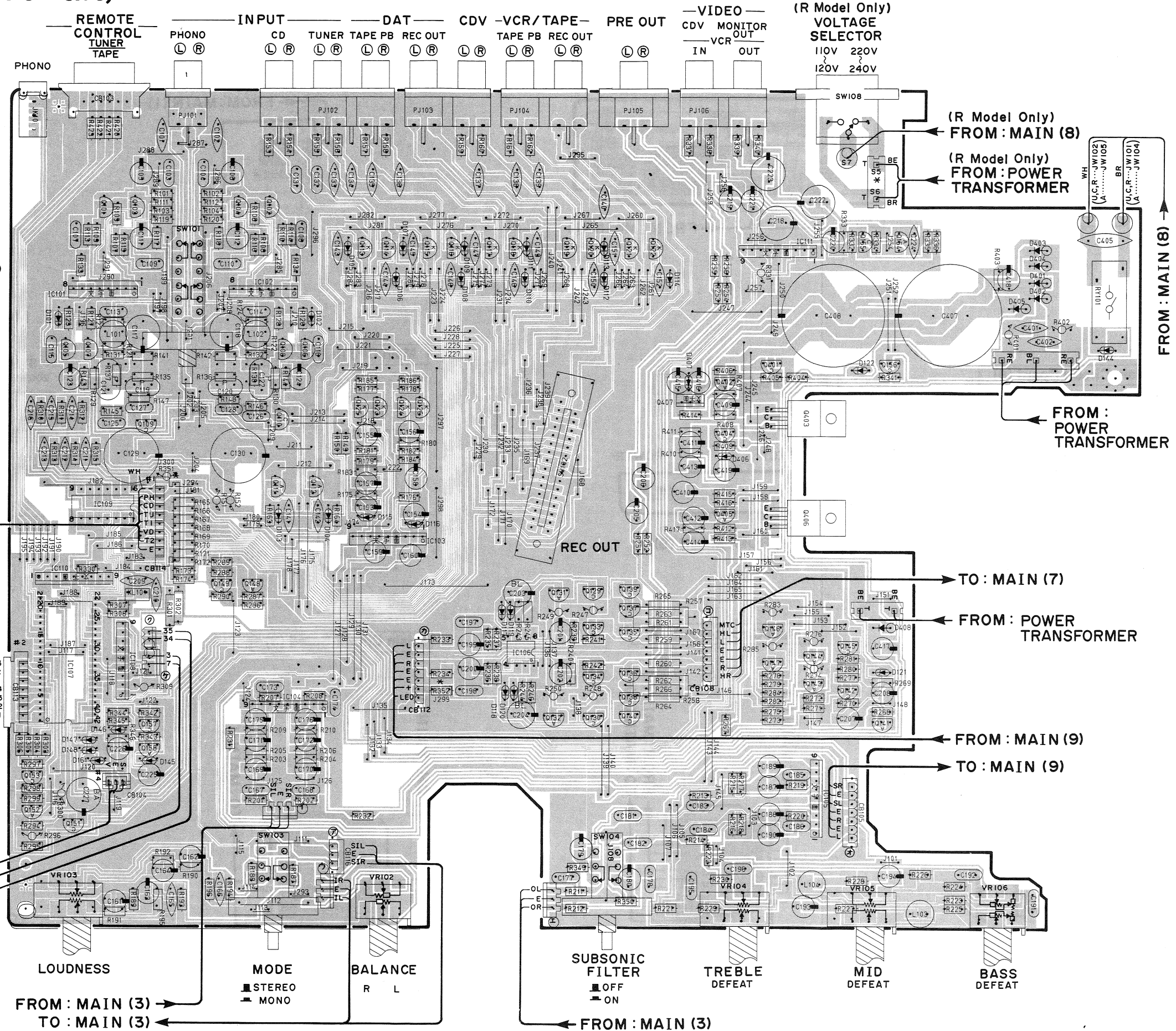
Main Circuit Board (1)
