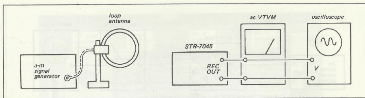
Fig. 3-8. A-m frequency coverage and tracking alignment test setup
