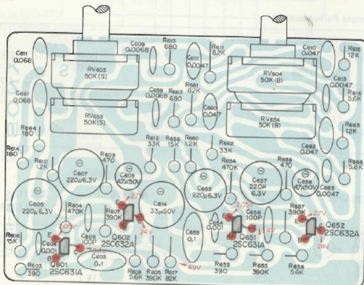
Transistor Location
