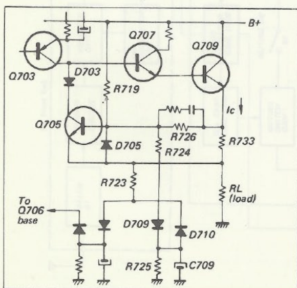
Fig. 1-2. Simplified protection circuit
