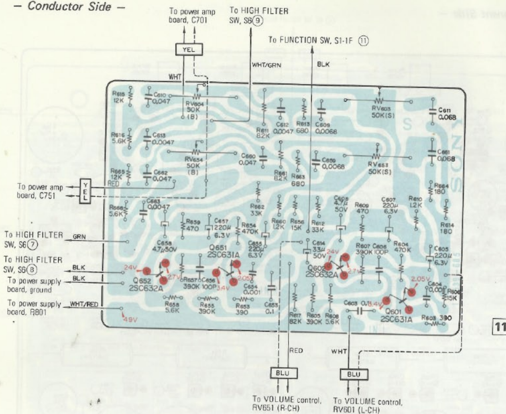
Transistor Location
