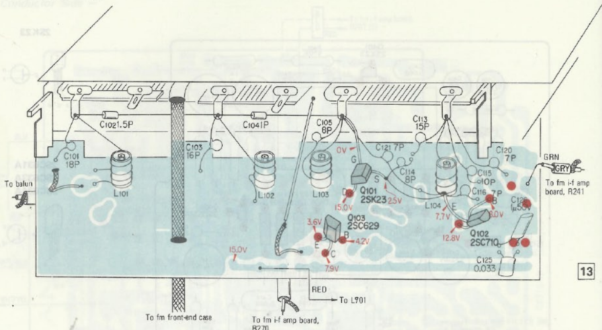
Transistor Location
