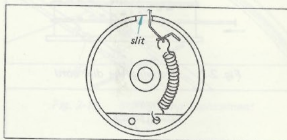
Fig. 2-6. Tension spring installation
