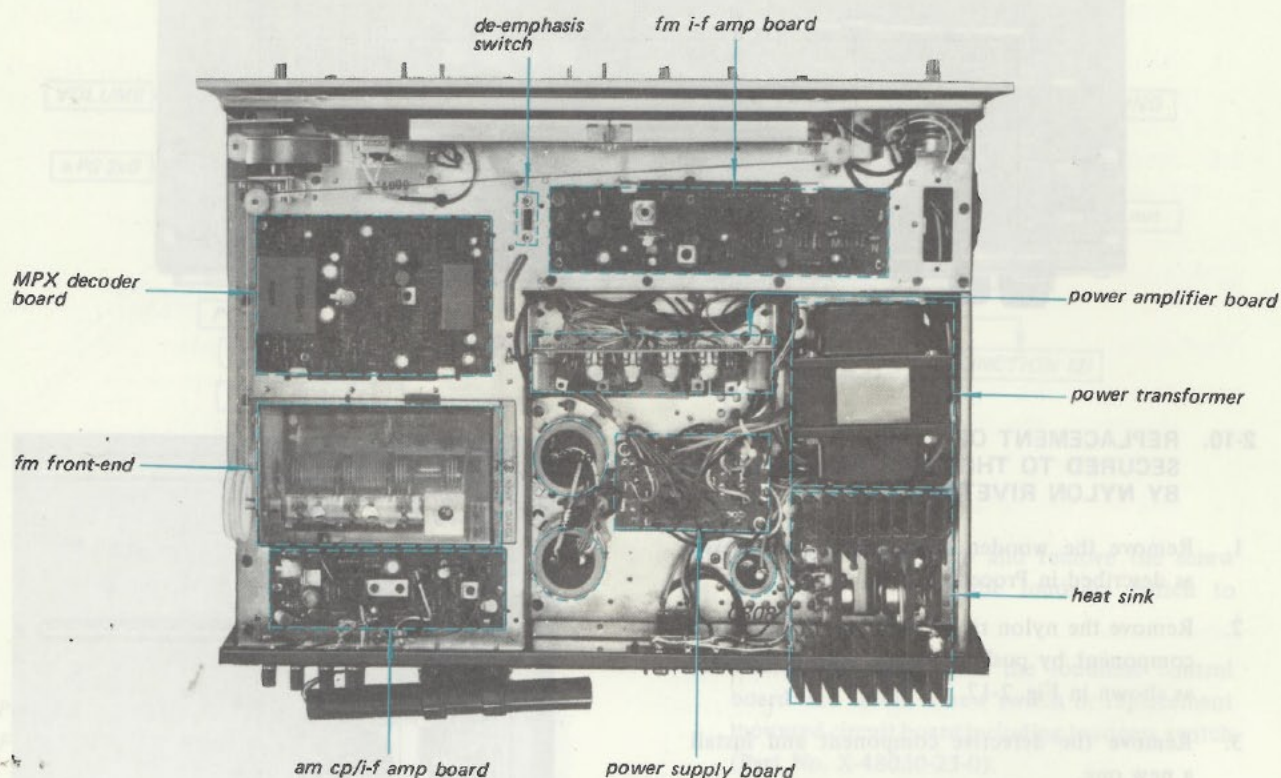
Fig. 2-19. Chassis top view
