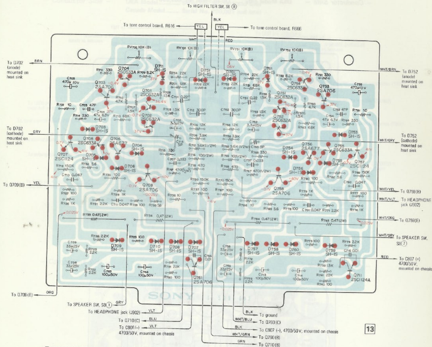
Transistors and Adjustment Parts Location
