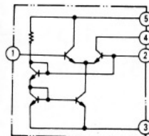
IC201 TA-7060(BA-401)
