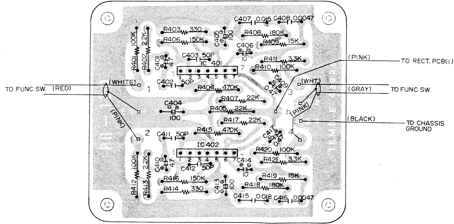
EQUALIZER AMPLIFIER CIRCUIT BOARD DIAGRAM
