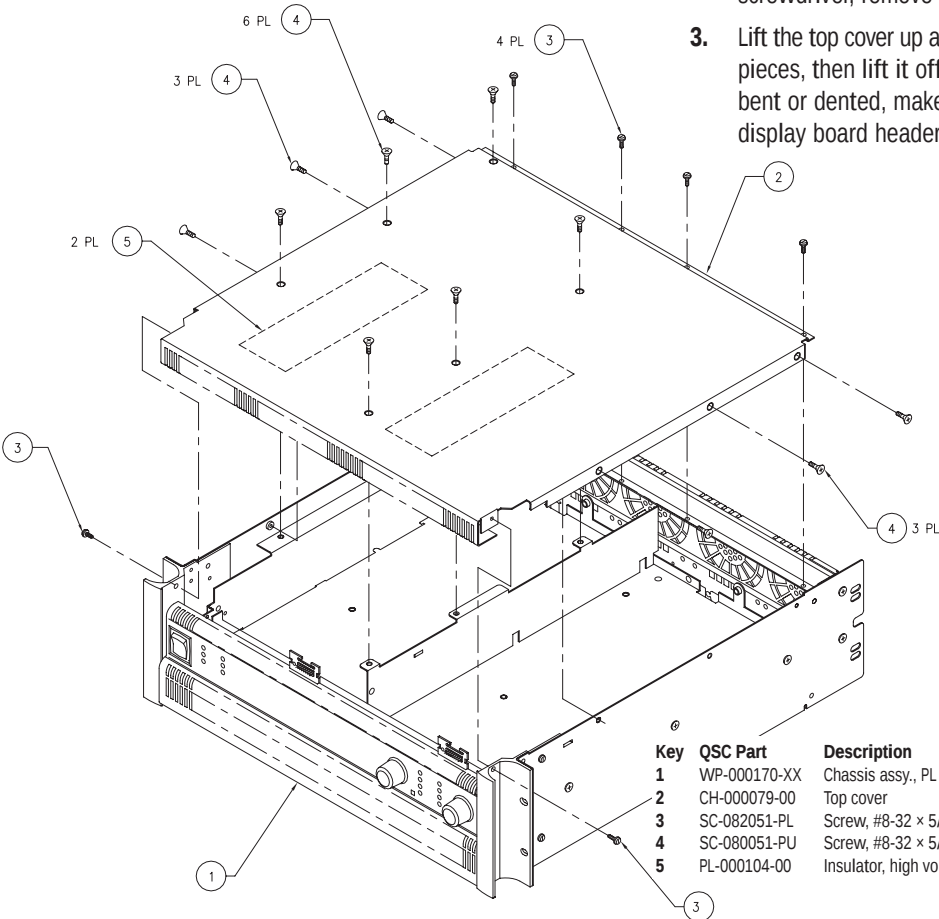
Figure 2.1. Removing or installing the top cover.
