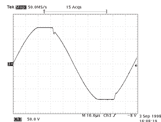
Figure 1.10. Most amps lose feedback during clipping, resulting in loss of damping and in “clip sticking.”
