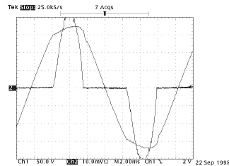
Figure 1.7. Amplifiers without PFC draw current only at the peaks of the AC voltage waveform.
