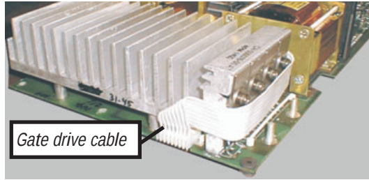
Figure 2.21. The gate drive cable for the MOSFETs. Disconnect it here for the V_{OUT} procedure.
