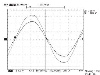
Figure 1.8. An amplifier with PFC draws current throughout the AC voltage waveform.
