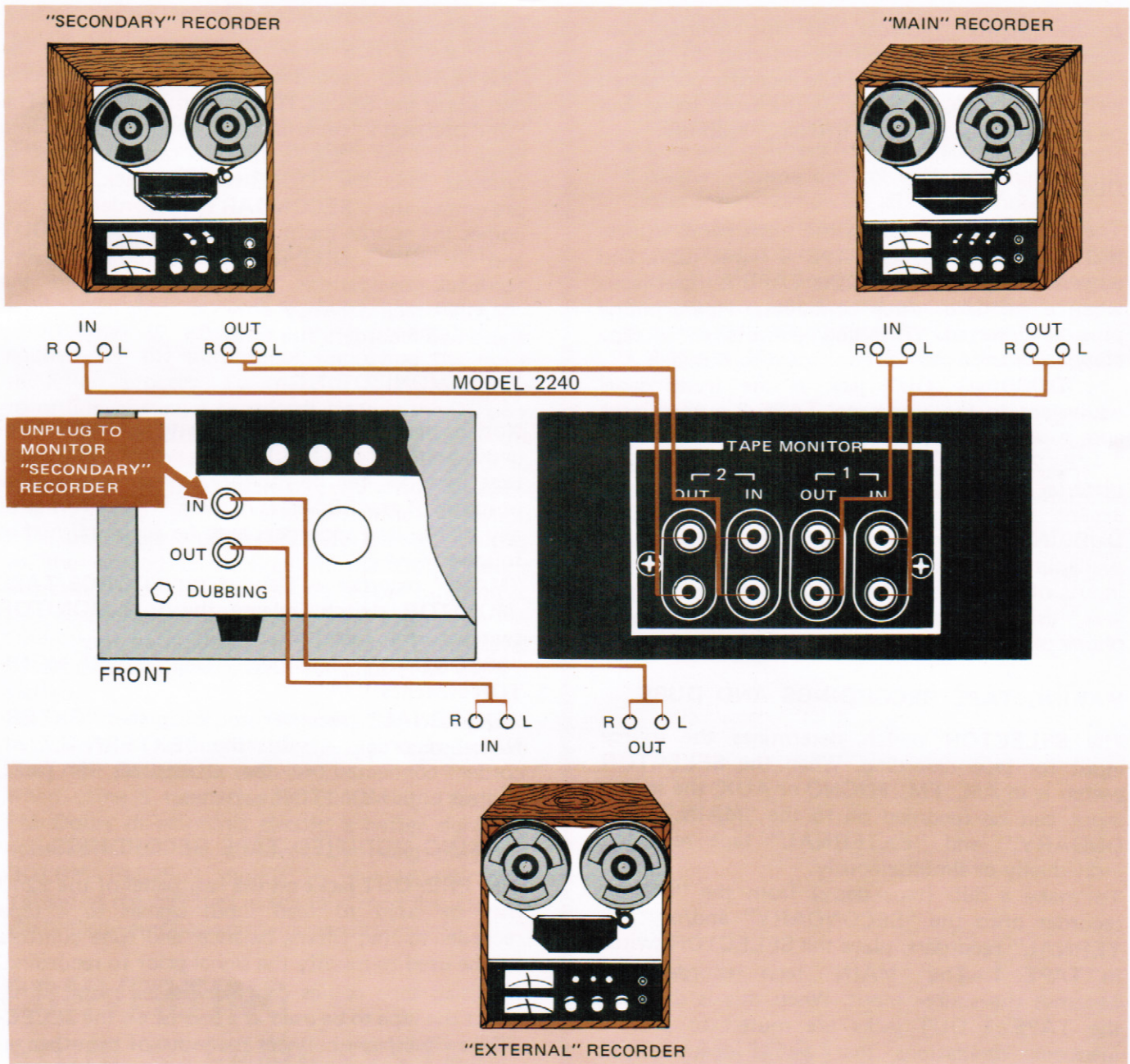
Figure 7. Tape Recorder Connections
