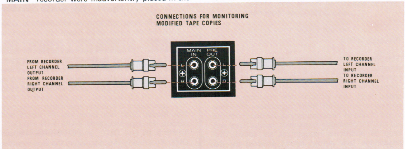
Figure 8. Arrangement for Making Modified Tape Copies
