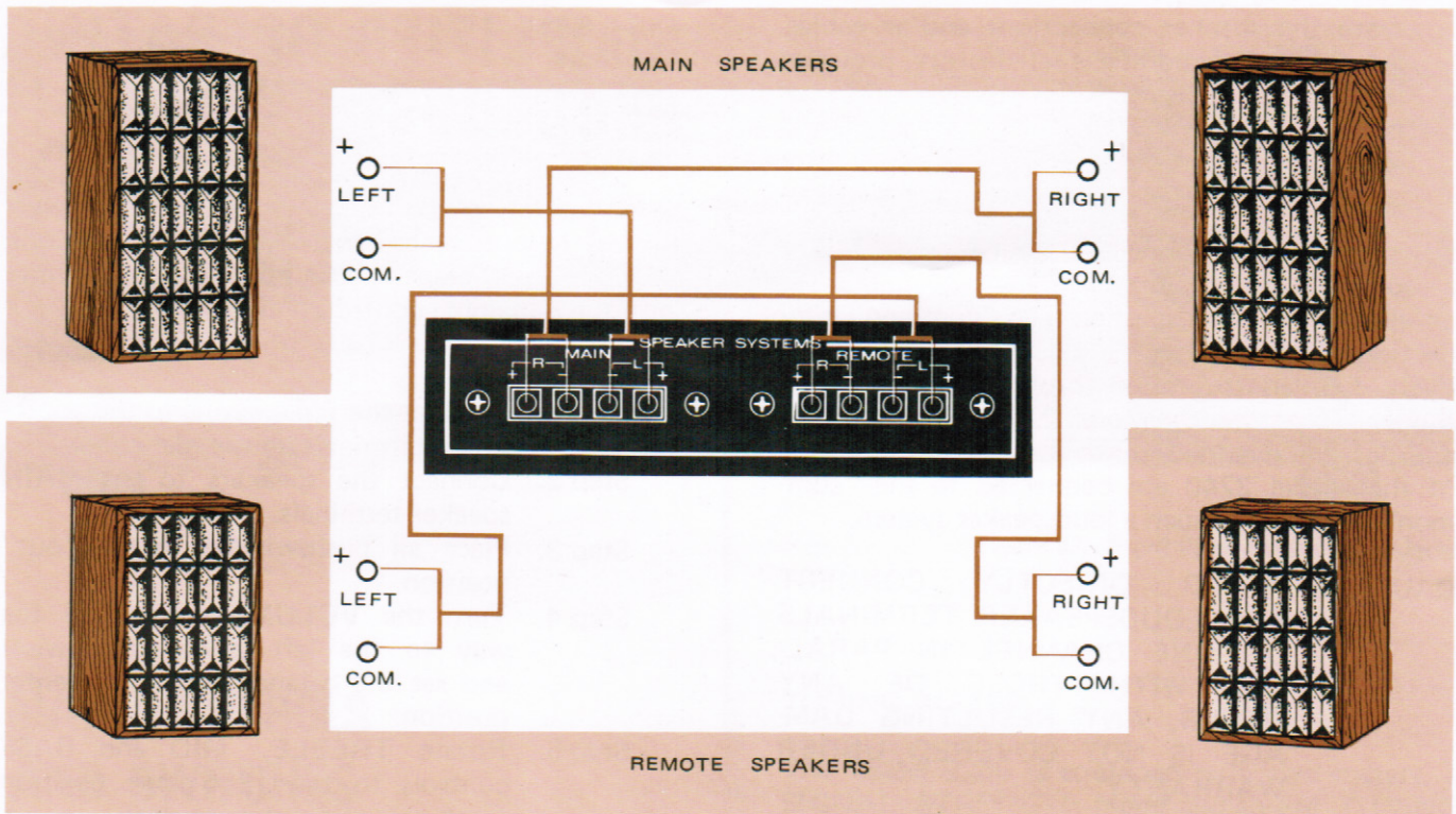
Figure 4. Speaker System Connections
