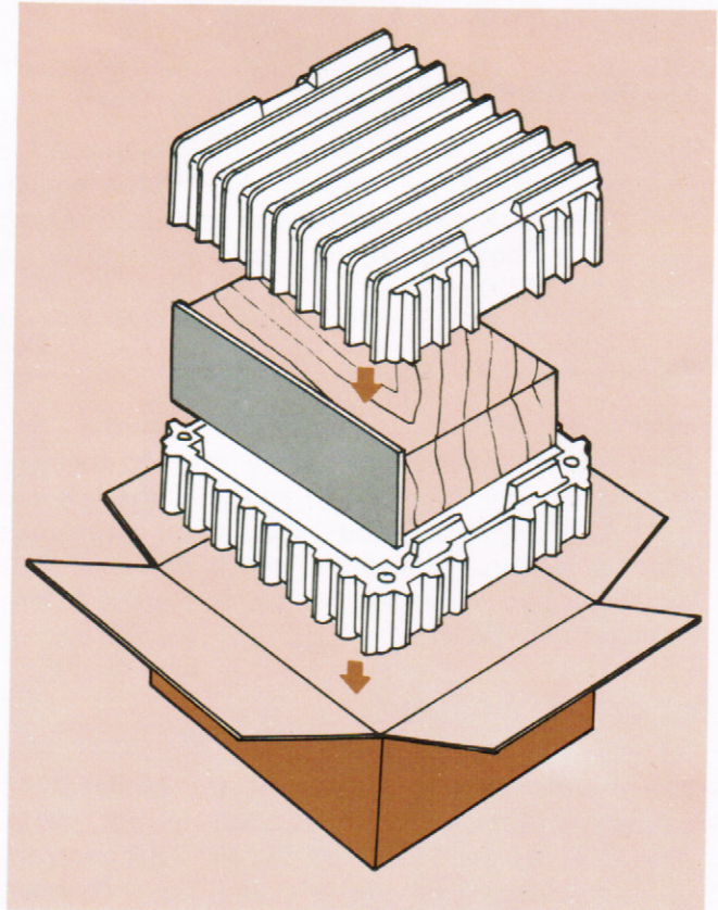
Figure 10. Packing Instructions
