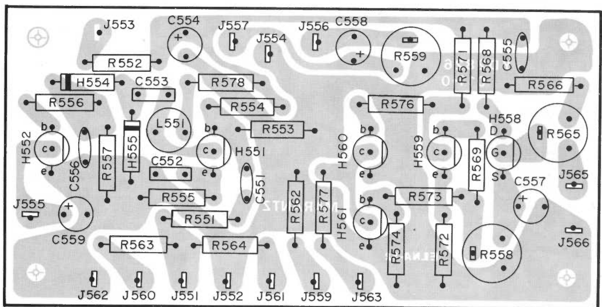
Figure 13. FM Noise and DC Amplifier Assembly P550 Component Locations
