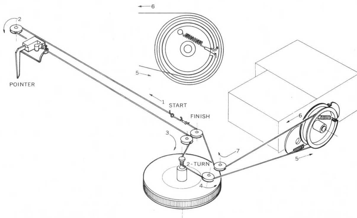
Figure 3. Dial Stringing
