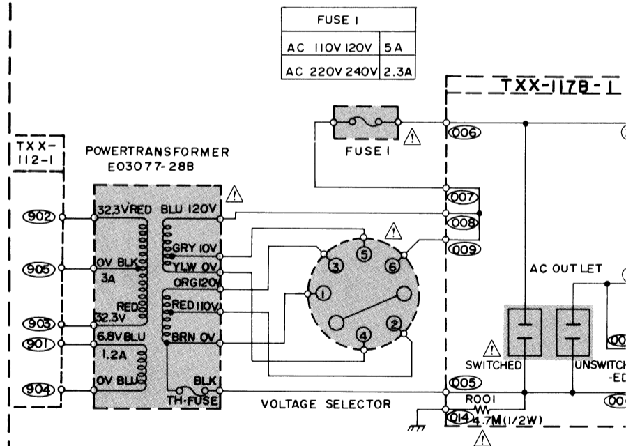
VOLTAGE SELECTOR CONNECTION
