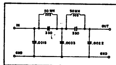
FILTER 024-1144-008 SCHEMATIC
