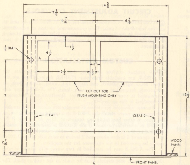
FIGURE 4. Top view of custom cabinet installation
