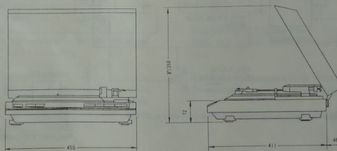
OUTER DIMENSIONS (mm)
