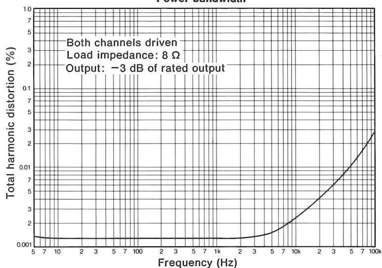
Power bandwidth
