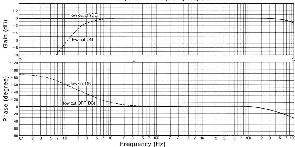
Gain and phase vs. frequency response
