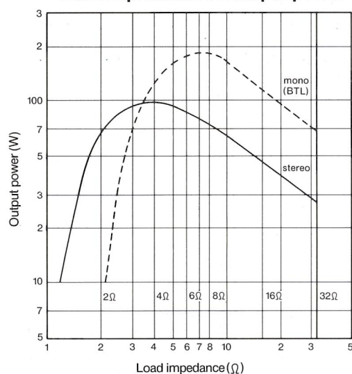
Load impedance vs. output power
