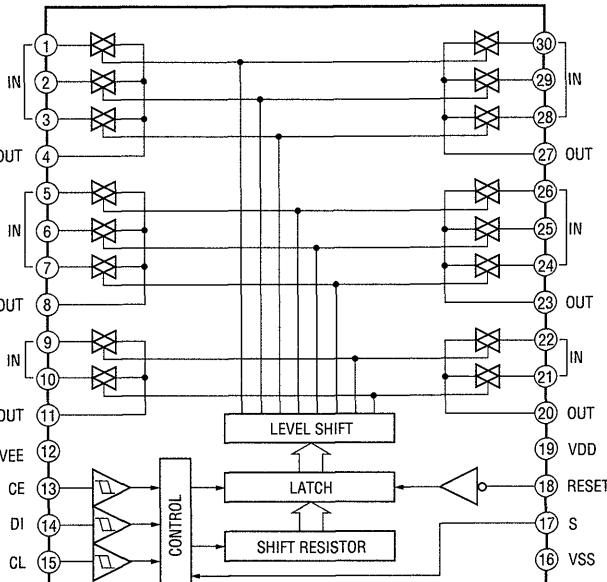
IC401, IC500 LC7822
