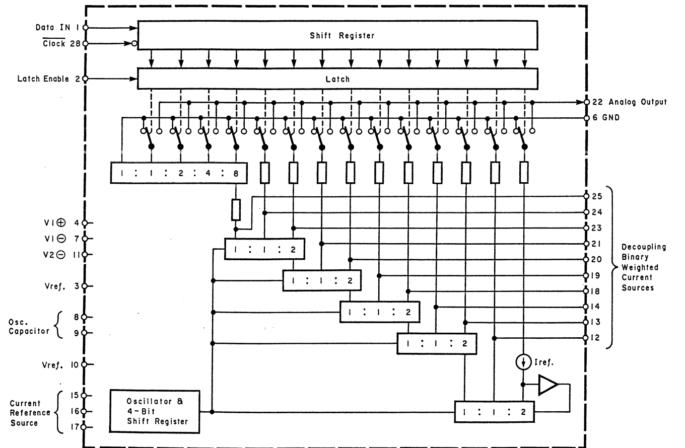
Fig. 8.1.22 D/A Converter IC TDA1540D
