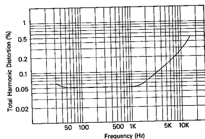
Frequency vs. Total Harmonic Distortion (Stereo)
