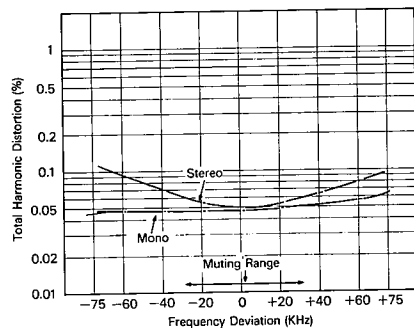
Frequency Deviation vs. Total Harmonic Distortion
