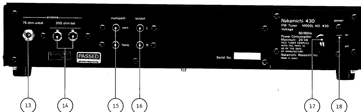
Fig. 1.2 Rear View
