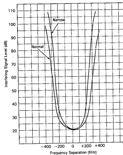
Selectivity
