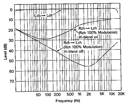
Stereo Separation
