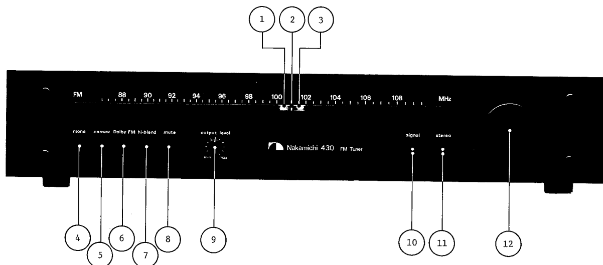
Fig. 1.1 Front View
