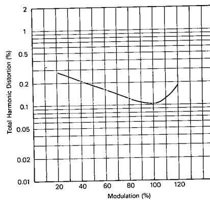
Modulation vs. Total Harmonic Distortion
