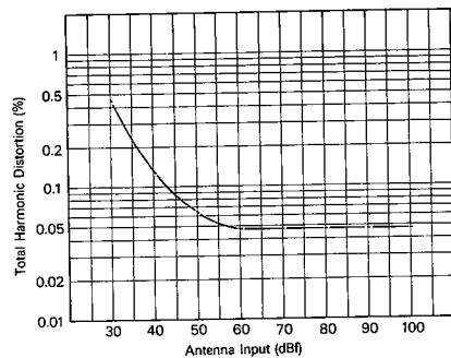
Input vs. Total Harmonic Distortion (Stereo)
