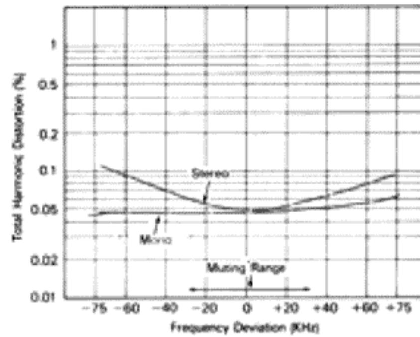
Frequency Deviation vs. Total Harmonic Distortion Antenna Input: 98MHz, 65dBf, 1mV, 300 Ohm Modulation: main 45.5% sub-carrier 45.5% pilot 9% AFC ON
