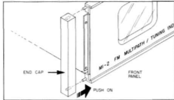
Figure 15. Fitting the End Caps to the Panel.
