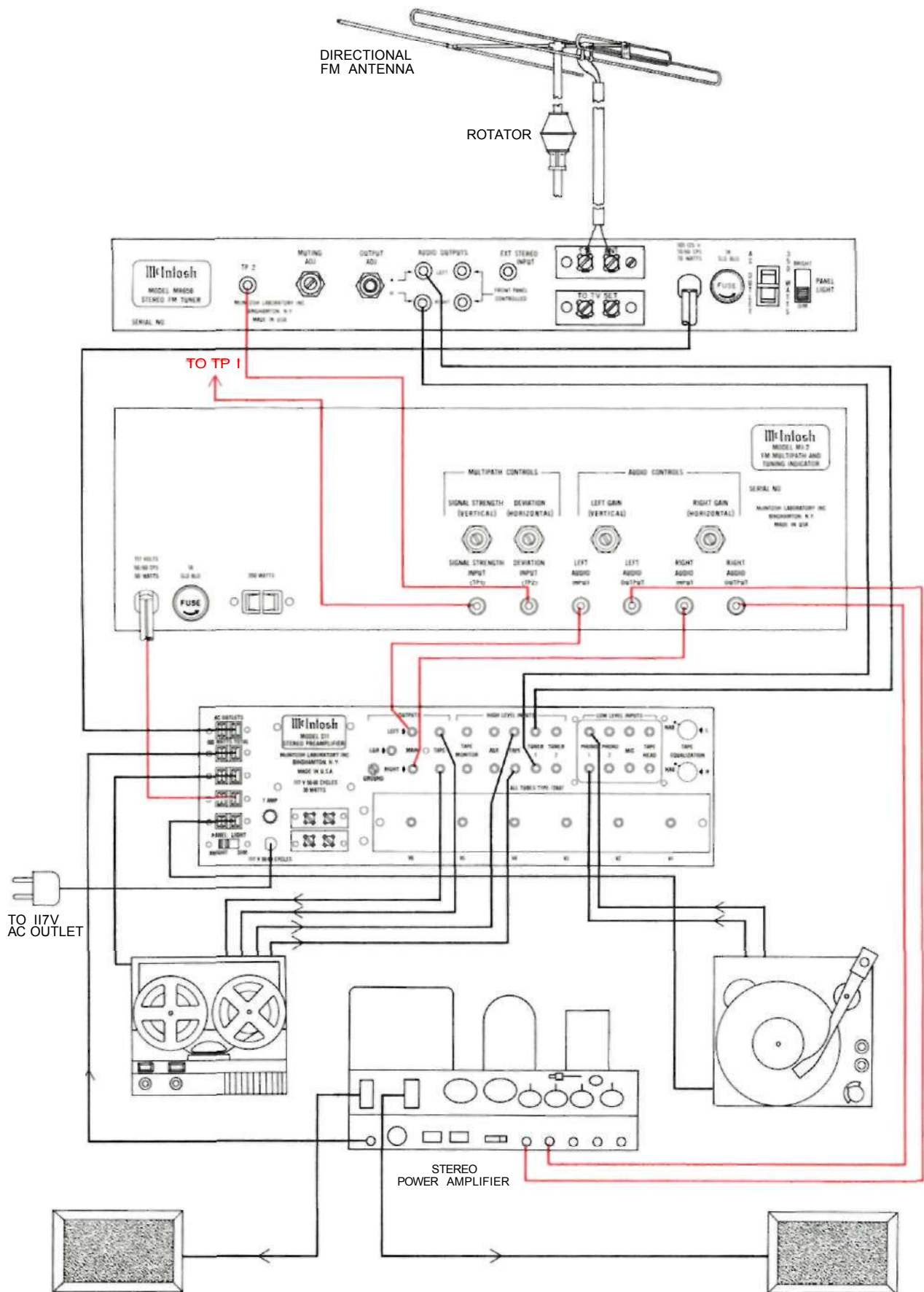
Figure 16. MI-2 Typical Hook-Up.
