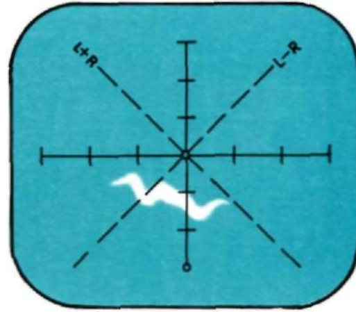
Figure 19. Irregular Pattern With Vertical Traces Indicating The Presence of Multipath.
