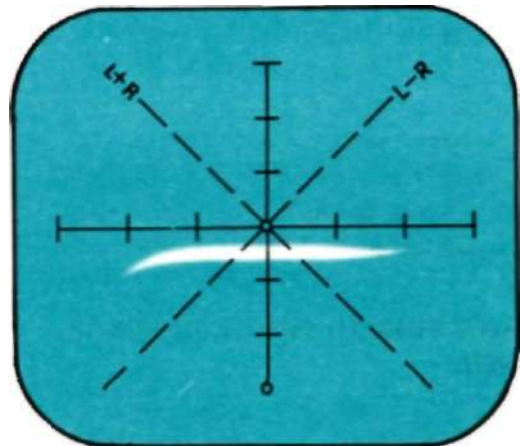
Figure 18. Uniform and Relatively Smooth Trace With Little or No Multipath Present (80% Modulation).
