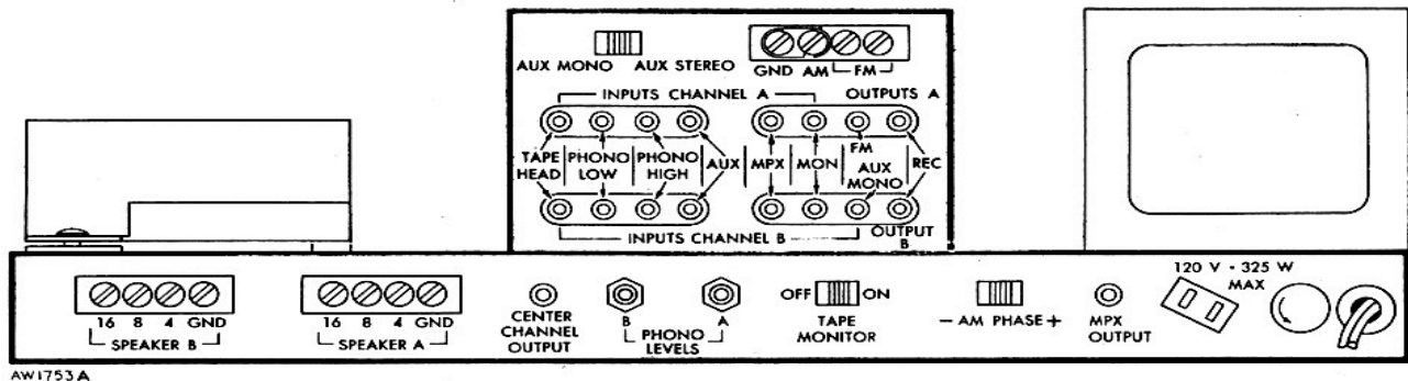
Figure 5. Rear panel.
