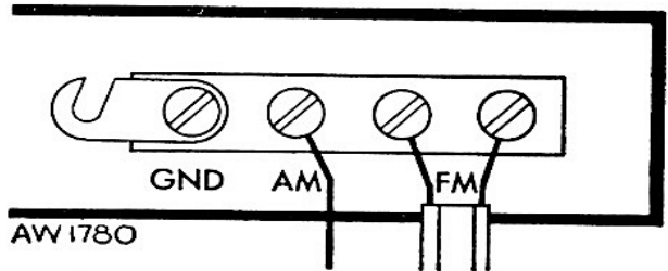
Figure 3. Connection of AM roof antenna (link must be detached).
