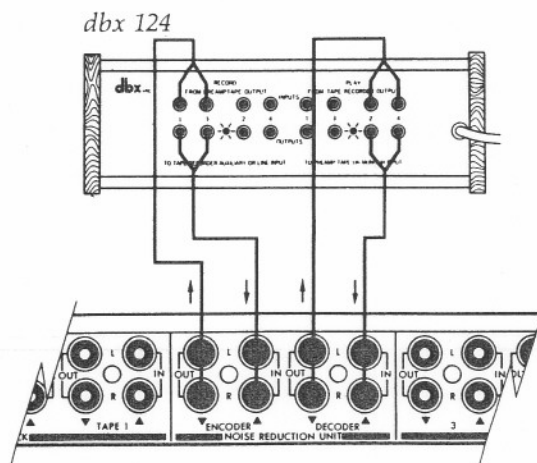
Figure 9: 124 hookup (note vacant jacks)
