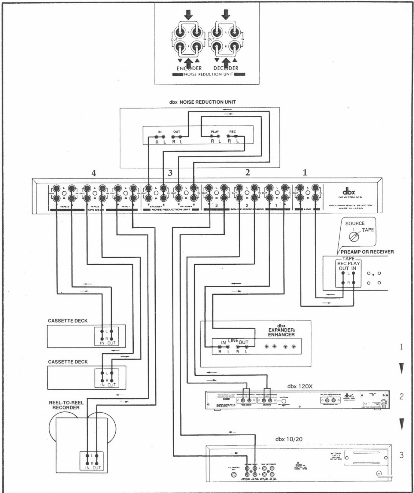
Figure 6: Hookups, by group
