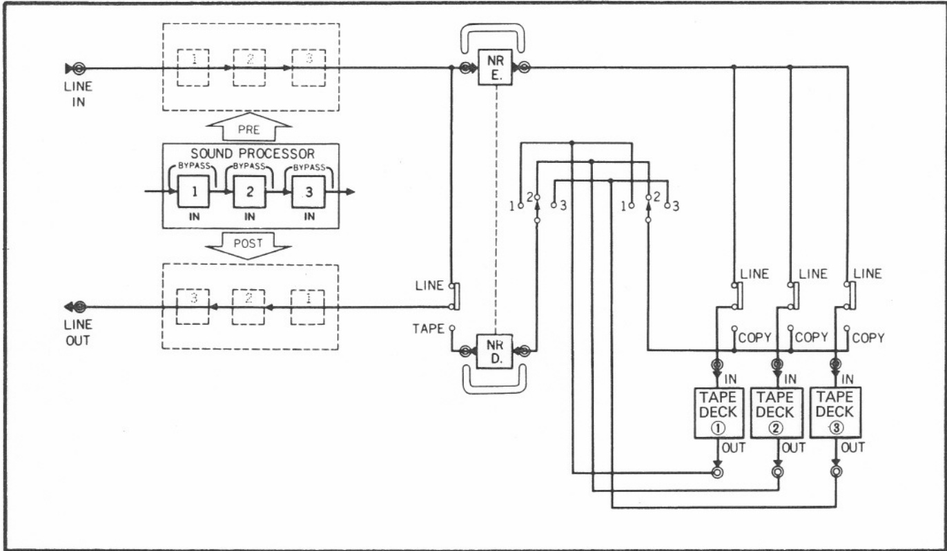
Figure 11: Block diagram of the model 200X
