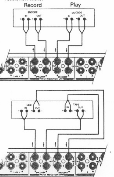
Examples of connections for non-dbx noise-reduction units.
