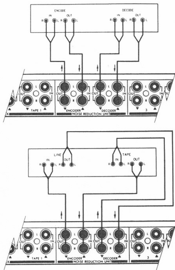
Figure 10: Examples of connections for non-dbx noise-reduction units. See text for various nomenclature.
