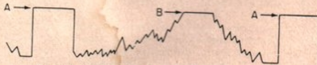
Figure 5—Overloaded or Clipped Video and Sync Signal.
