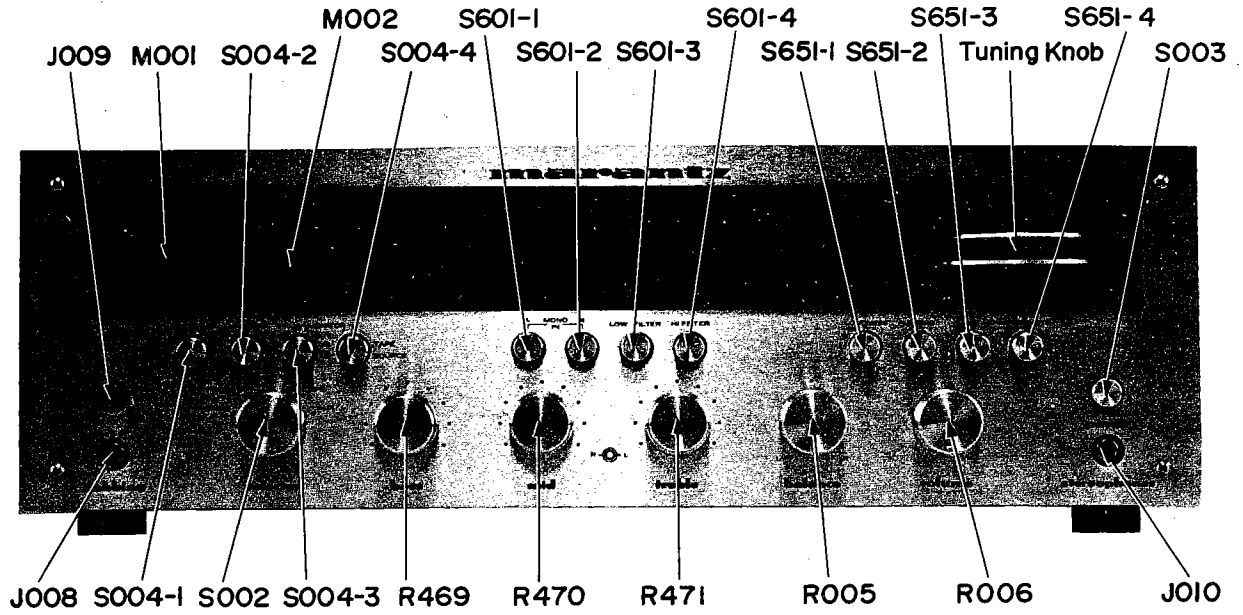
Figure 5 Front Panel Adjustment and Component Locations
