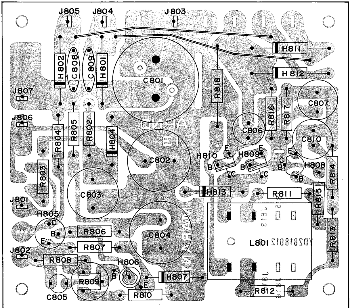
Figure 19 Regulated Power Supply and Protection Relay Circuit Assembly P800 Component Locations
