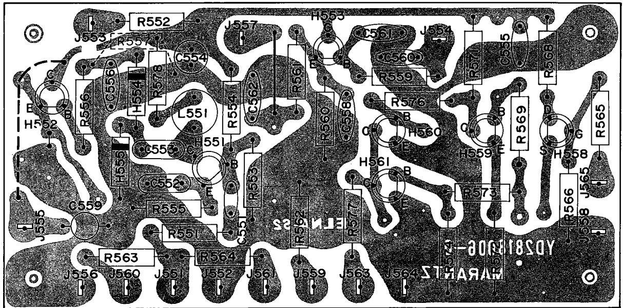
Figure 13 Muting Control Amplifier Assembly P550 Component Locations
