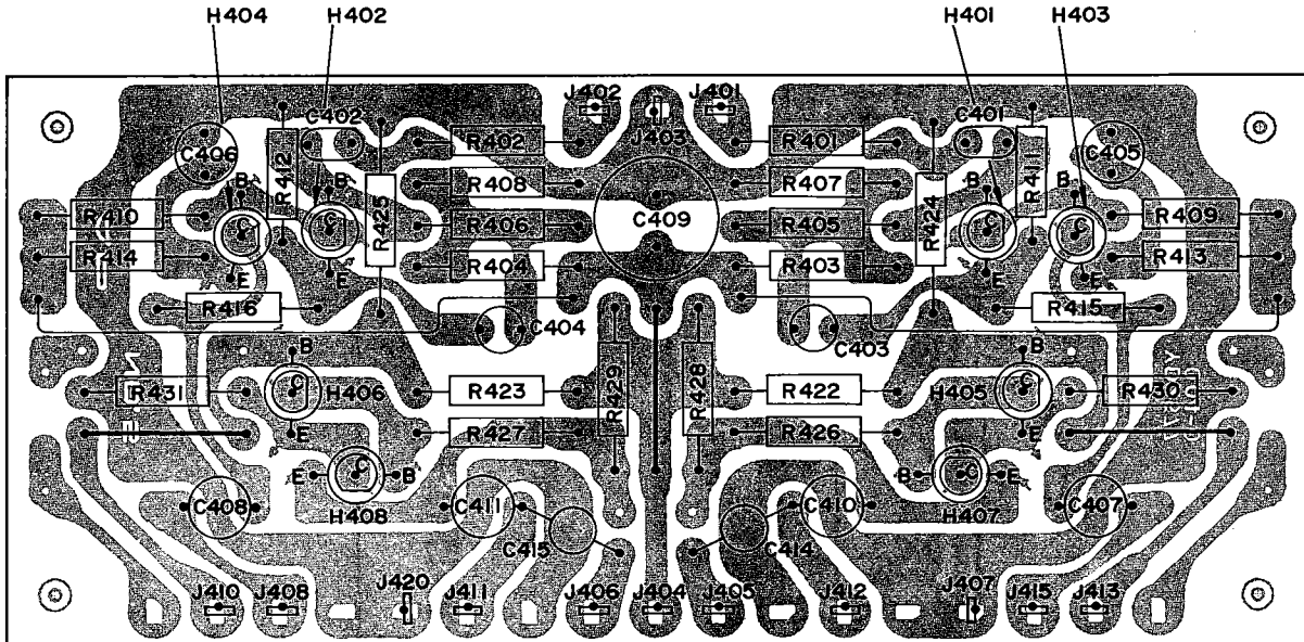
Figure 16 Tone Amplifier Assembly P400 Component Locations
